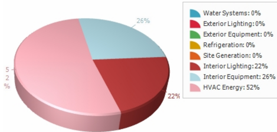
Total Site Energy Breakdown
