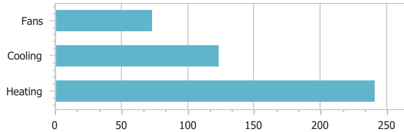
HVAC Energy Usage
