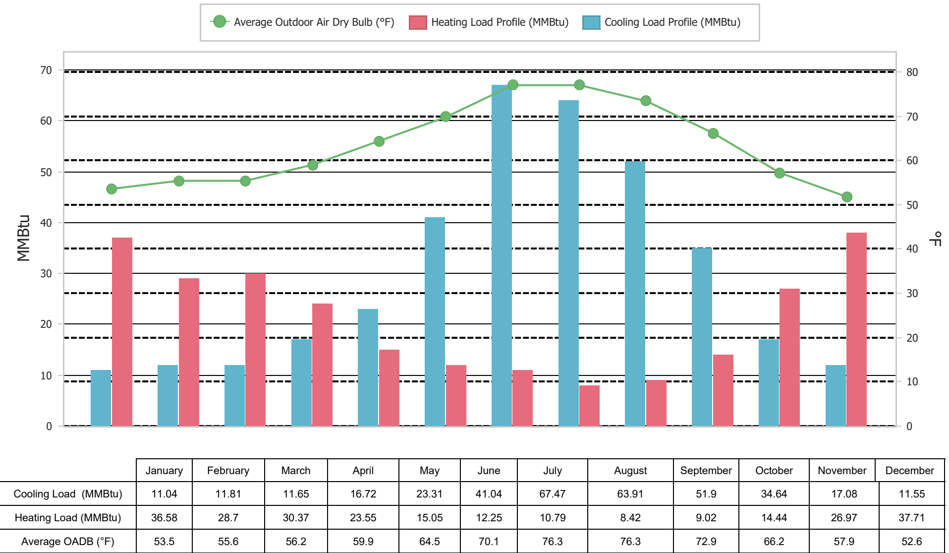
Site HVAC Load Profile
