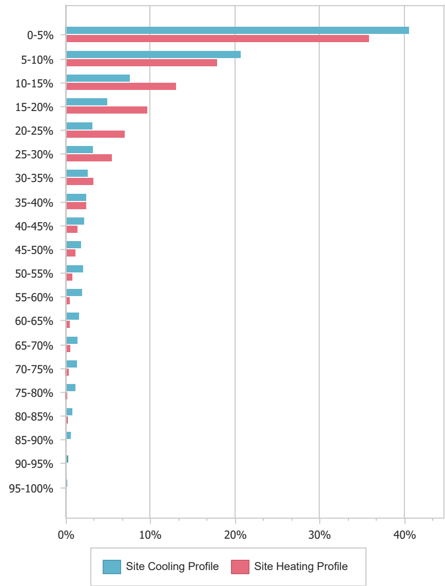
Site HVAC Hourly Load Distribution
