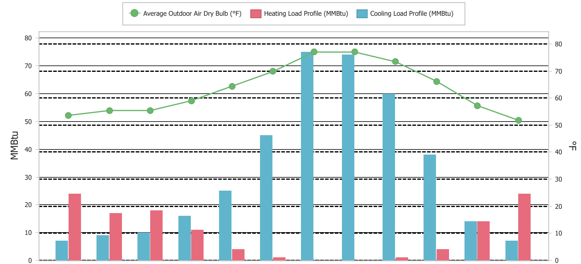
Site HVAC Load Profile
